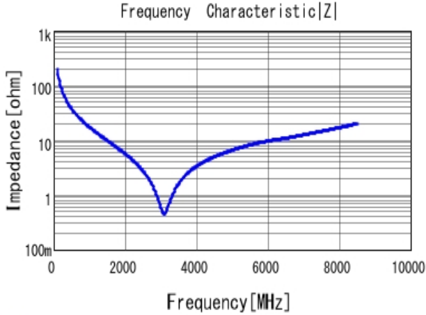
■ GRM1555C1H8R2BA01 |Z| DCOV, 25degC
