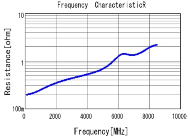
■ GRM1555C1H8R2BA01 R DCOV, 25degC
