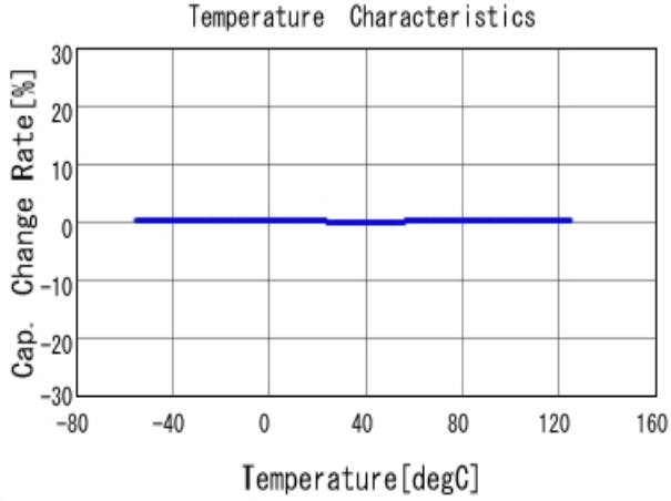
■ GRM1555C1H8R2BA01 C-Temp. capchange, DCOV, AC1Vrms
