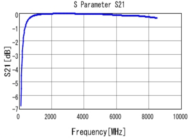
■ GRM1555C1H8R2BA01 S21 DCOV, 25degC
