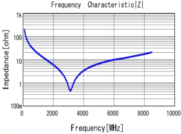
■ GRM1555C1H8R0DA01 |Z| DCOV, 25degC
