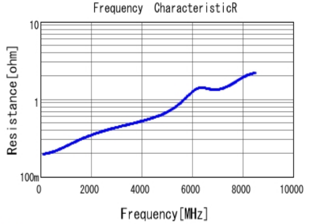
■ GRM1555C1H8R0DA01 R DCOV, 25degC
