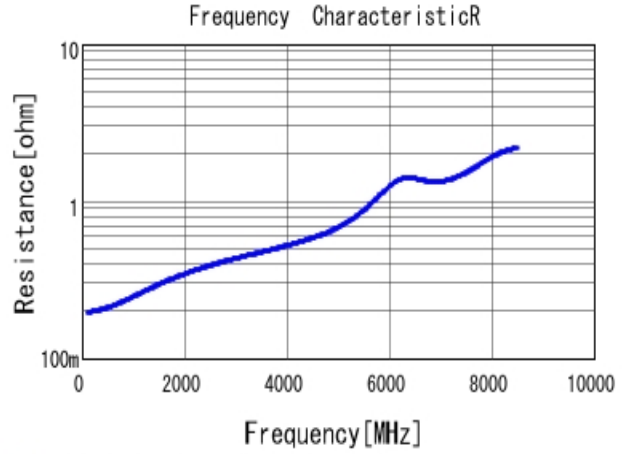
■ GRM1555C1H8R0CA01 R DCOV, 25degC
