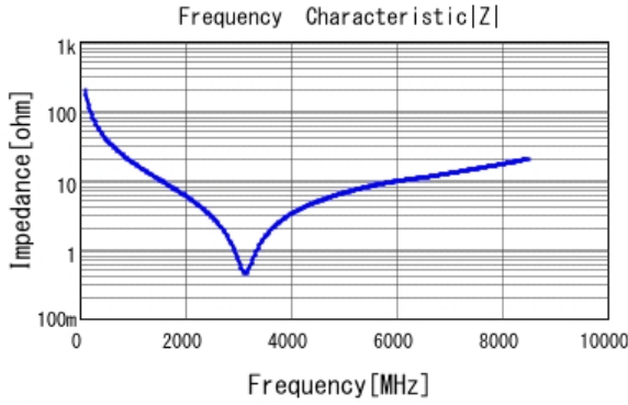
■ GRM1555C1H8R0BA01 |Z| DCOV, 25degC
