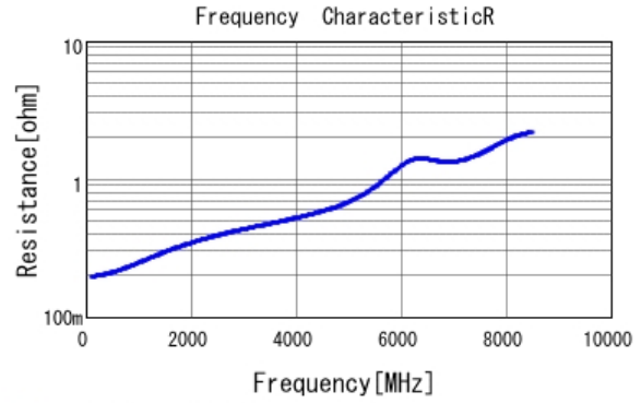
■ GRM1555C1H8R0BA01 R DCOV, 25degC
