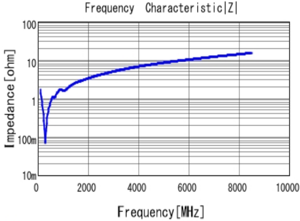
■ GRM1555C1H821JA01 |Z| DCOV, 25degC
