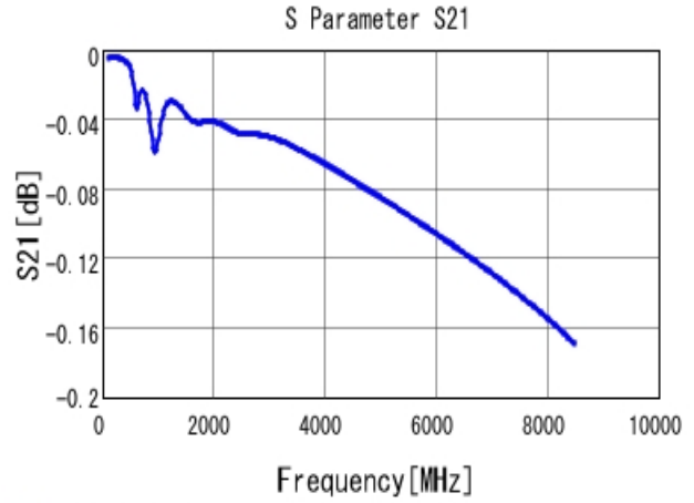
■ GRM1555C1H821JA01 S21 DCOV, 25degC
