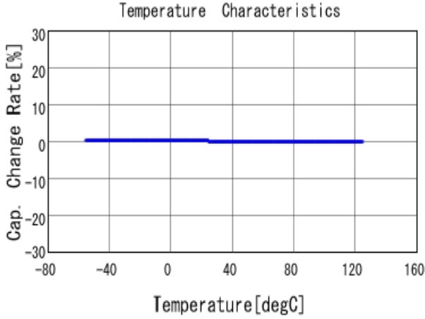
■ GRM1555C1H820GA01 C-Temp. capchange, DCOV, AC1Vrms
