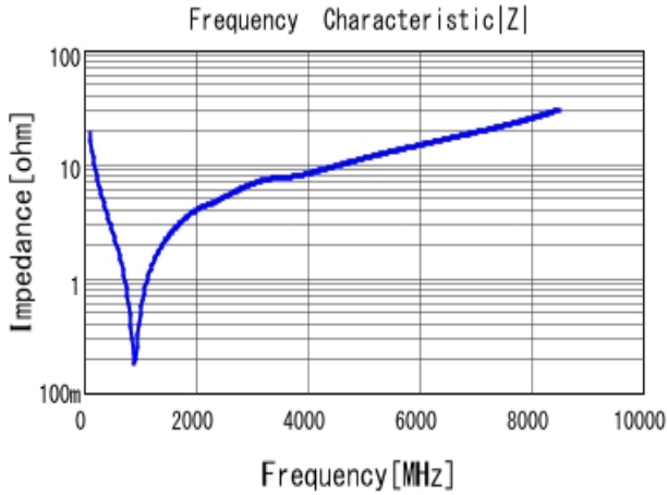
■ GRM1555C1H820GA01 |Z| DCOV, 25degC
