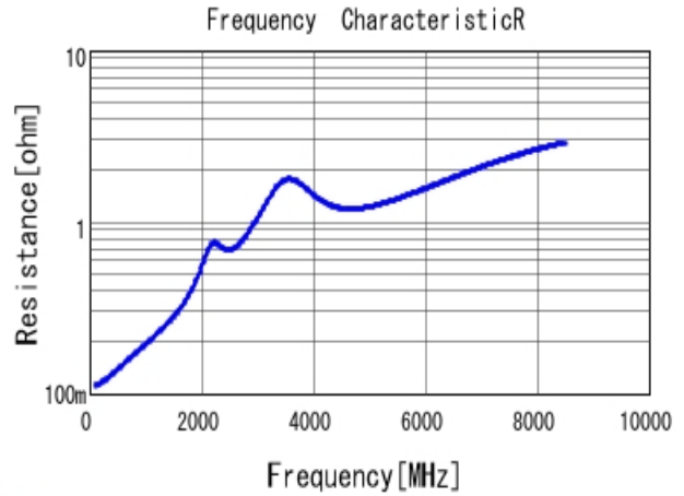
■ GRM1555C1H820GA01 R DCOV, 25degC
