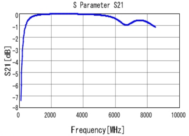
■ GRM1555C1H7R5DA01 S21 DCOV, 25degC
