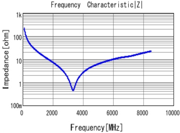
■ GRM1555C1H7R0DA01 |Z| DCOV, 25degC
