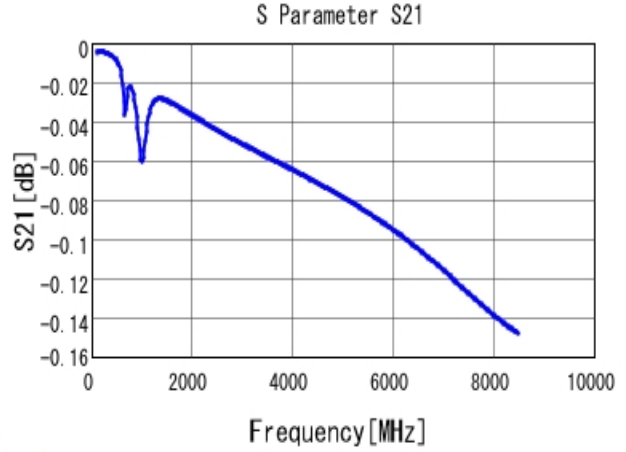
■ GRM1555C1H751GA01 S21 DCOV, 25degC
