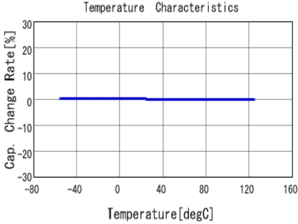
■ GRM1555C1H751GA01 C-Temp. capchange, DCOV, AC1Vrms
