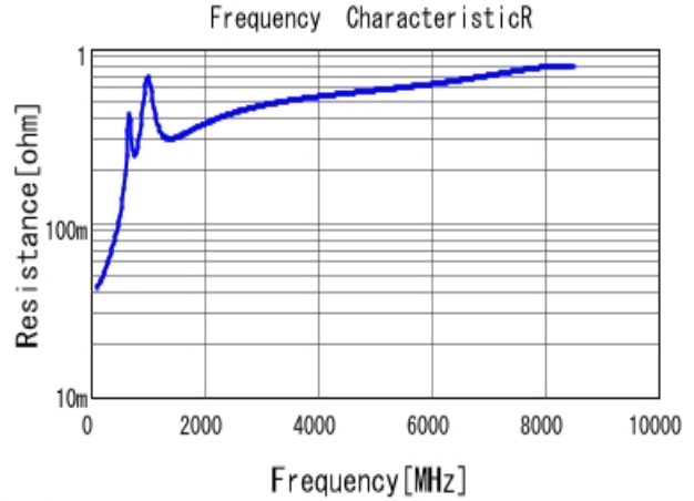
■ GRM1555C1H751GA01 R DCOV, 25degC
