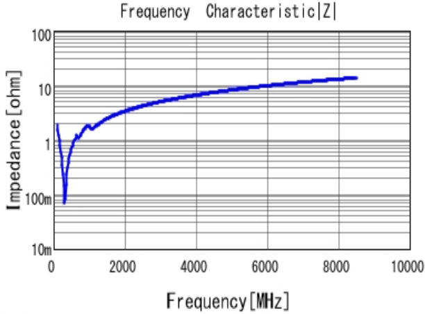
■ GRM1555C1H751GA01 |Z| DCOV, 25degC
