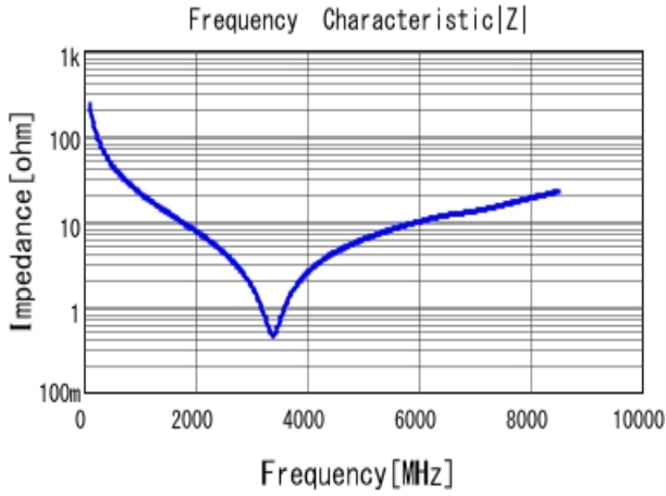
■ GRM1555C1H6R8CA01 |Z| DCOV, 25degC
