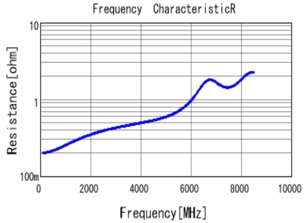
■ GRM1555C1H6R8CA01 R DCOV, 25degC
