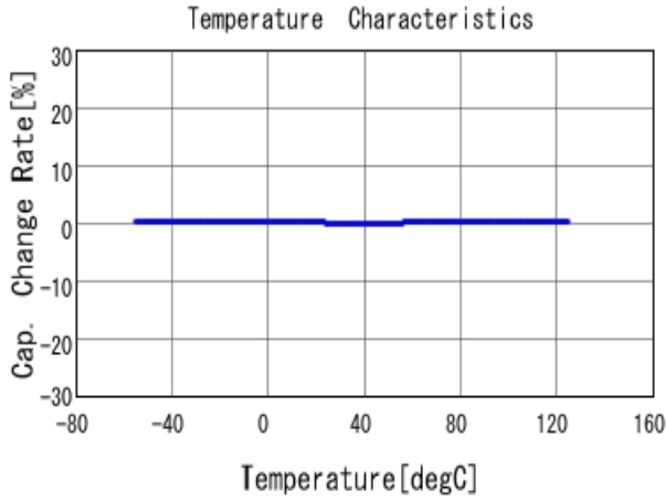
■ GRM1555C1H6R8CA01 C-Temp. capchange, DCOV, AC1Vrms
