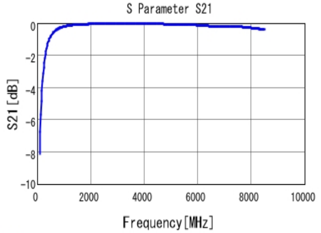
■ GRM1555C1H6R8CA01 S21 DCOV, 25degC
