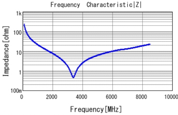
■ GRM1555C1H6R8BA01 |Z| DCOV, 25degC
