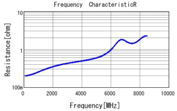
■ GRM1555C1H6R8BA01 R DCOV, 25degC
