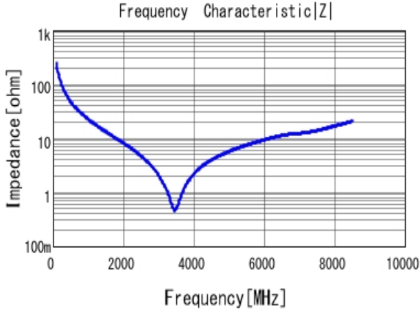
■ GRM1555C1H6R5CA01 |Z| DCOV, 25degC
