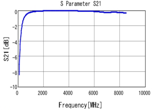
■ GRM1555C1H6R5CA01 S21 DCOV, 25degC
