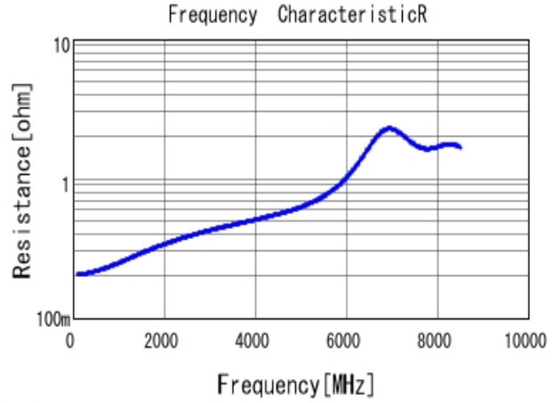
■ GRM1555C1H6R5CA01 R DCOV, 25degC
