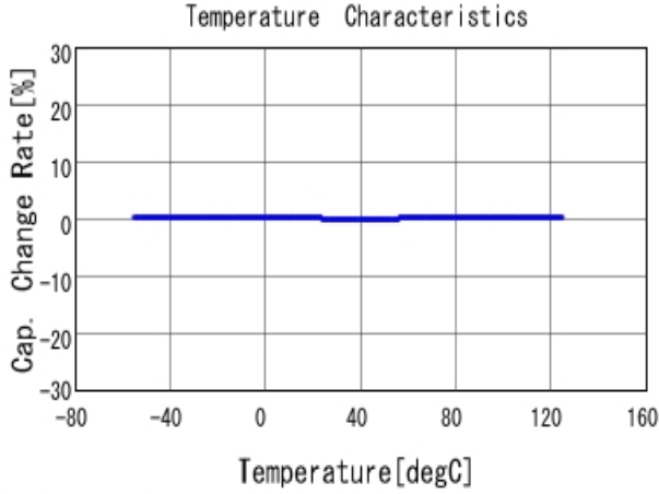
■ GRM1555C1H6R5CA01 C-Temp. capchange, DCOV, AC1Vrms
