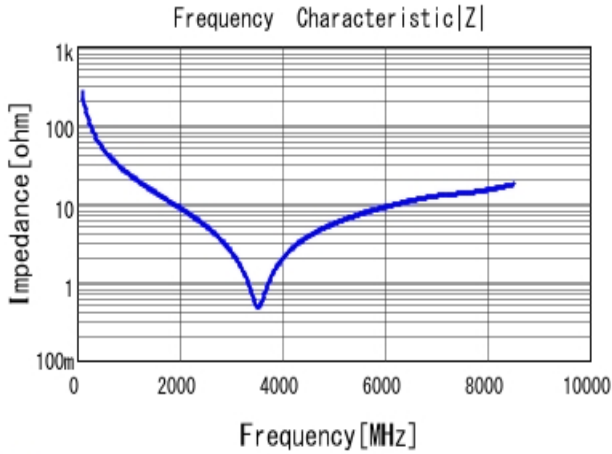
■ GRM1555C1H6R2WA01 |Z| DCOV, 25degC
