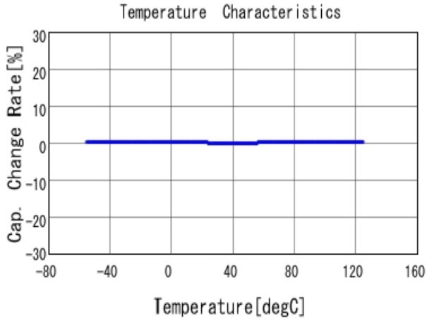
■ GRM1555C1H6R2WA01 C-Temp. capchange, DCOV, AC1Vrms
