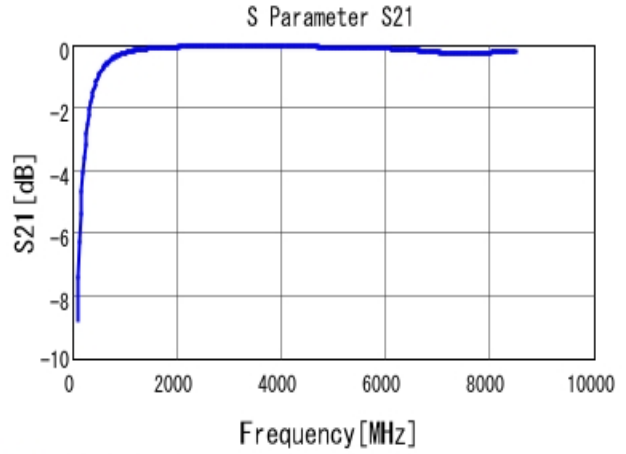
■ GRM1555C1H6R2WA01 S21 DCOV, 25degC
