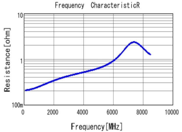
■ GRM1555C1H6R2WA01 R DCOV, 25degC
