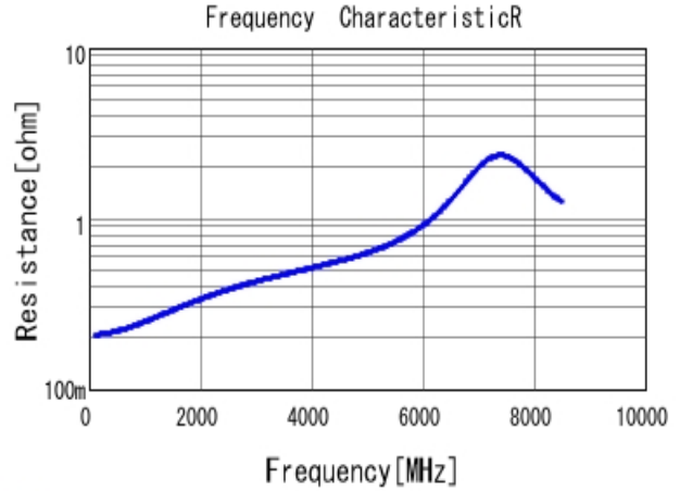
■ GRM1555C1H6R2CA01 R DCOV, 25degC
