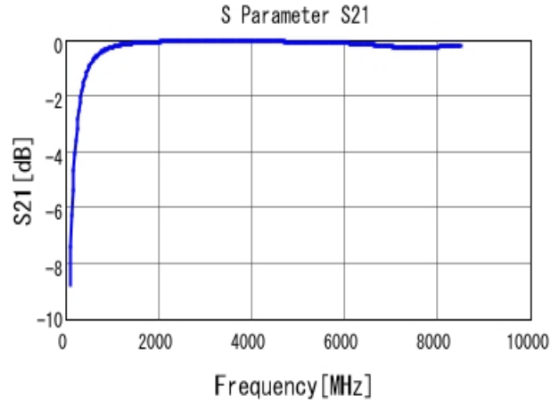
■ GRM1555C1H6R2CA01 S21 DCOV, 25degC
