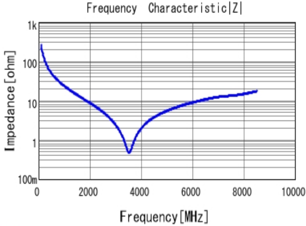
■ GRM1555C1H6R2CA01 |Z| DCOV, 25degC
