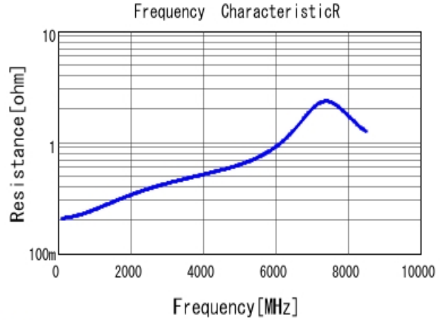
■ GRM1555C1H6R2BA01 R DCOV, 25degC
