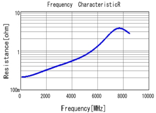
■ GRM1555C1H6R0DA01 R DCOV, 25degC
