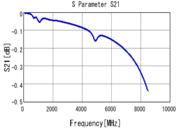
■ GRM1555C1H681JA01 S21 DCOV, 25degC
