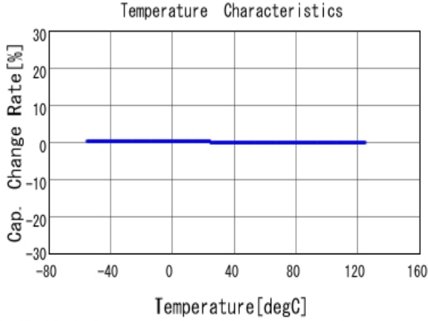
■ GRM1555C1H681JA01 C-Temp. capchange, DCOV, AC1Vrms
