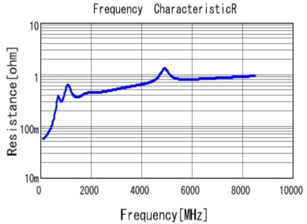
■ GRM1555C1H681JA01 R DCOV, 25degC
