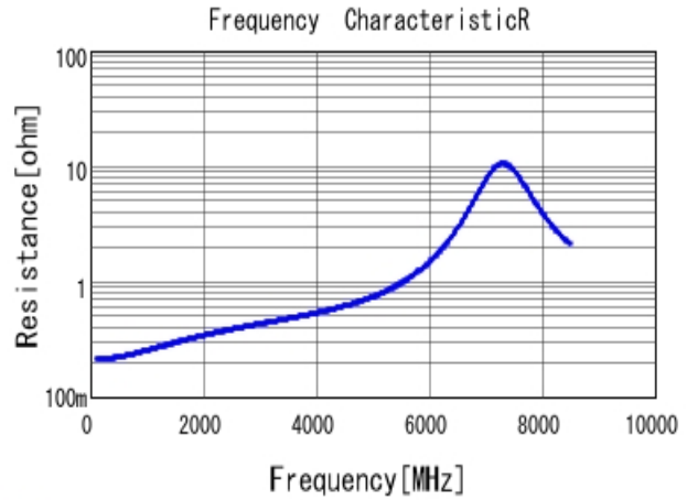
■ GRM1555C1H5R6DA01 R DCOV, 25degC
