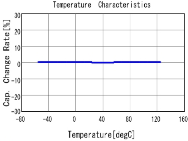
■ GRM1555C1H5R6DA01 C-Temp. capchange, DCOV, AC1Vrms
