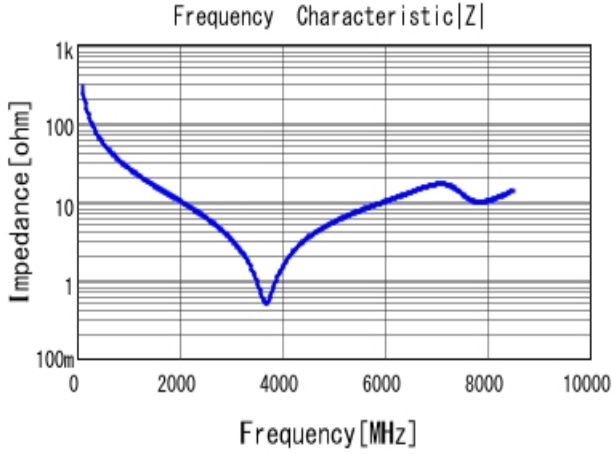
■ GRM1555C1H5R6BA01 |Z| DCOV, 25degC
