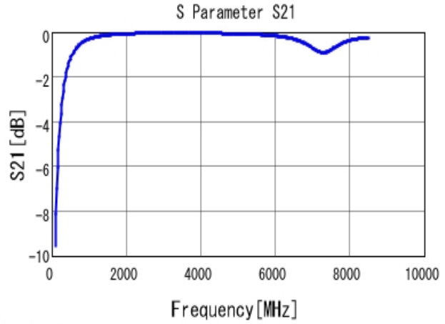
■ GRM1555C1H5R6BA01 S21 DCOV, 25degC
