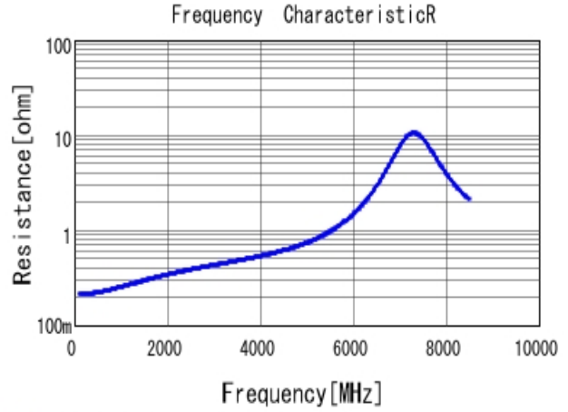
■ GRM1555C1H5R6BA01 R DCOV, 25degC
