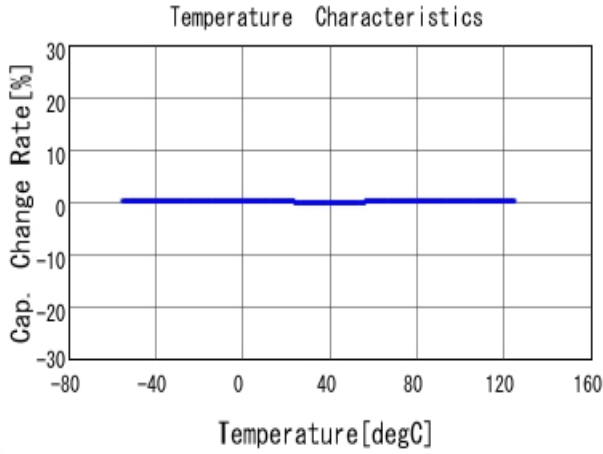
■ GRM1555C1H5R6BA01 C-Temp. capchange, DCOV, AC1Vrms
