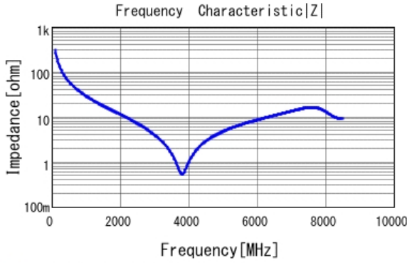
■ GRM1555C1H5R1CA01 |Z| DCOV, 25degC
