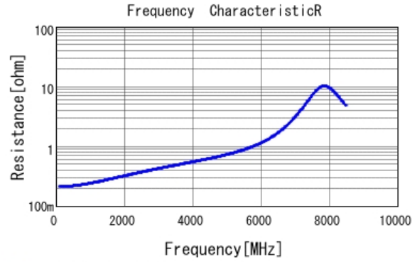
■ GRM1555C1H5R1CA01 R DCOV, 25degC
