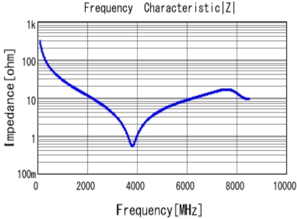
■ GRM1555C1H5R1BA01 |Z| DC0V, 25degC
