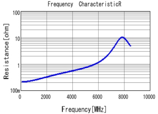
■ GRM1555C1H5R1BA01 R DC0V, 25degC
