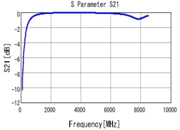
■ GRM1555C1H5R1BA01 S21 DCOV, 25degC
