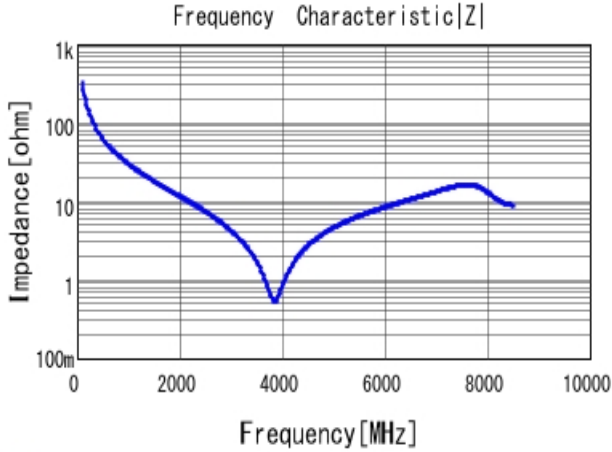
■ GRM1555C1H5R0BA01 |Z| DC0V, 25degC
