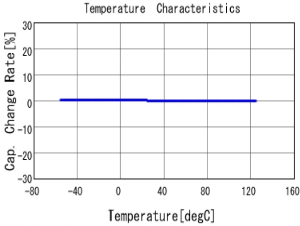
■ GRM1555C1H560JA01 C-Temp. capchange, DCOV, AC1Vrms
