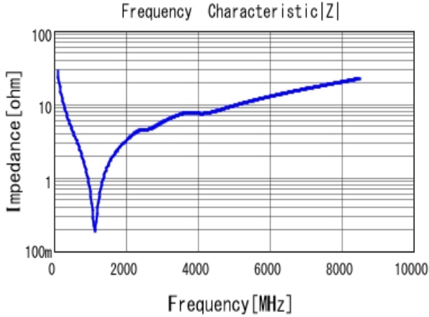
■ GRM1555C1H560JA01 |Z| DC0V, 25degC
