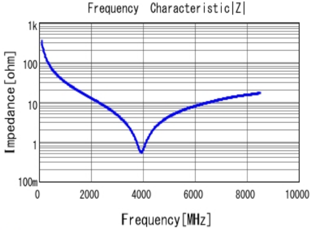
■ GRM1555C1H4R7BA01 |Z| DC0V, 25degC
