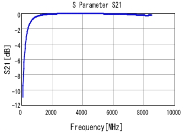
■ GRM1555C1H4R7BA01 S21 DCOV, 25degC
