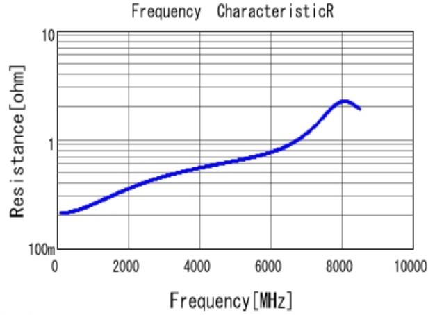
■ GRM1555C1H4R7BA01 R DC0V, 25degC
