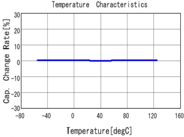
■ GRM1555C1H4R3CA01 C-Temp. capchange, DCOV, AC1Vrms
