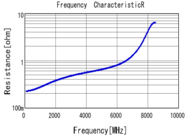
■ GRM1555C1H4R3CA01 R DC0V, 25degC
