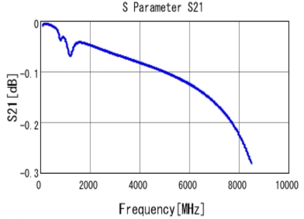
■ GRM1555C1H471JA01 S21 DCOV, 25degC
