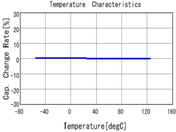
■ GRM1555C1H471JA01 C-Temp. capchange, DCOV, AC1Vrms
