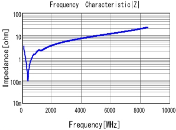
■ GRM1555C1H471GA01 |Z| DCOV, 25degC
