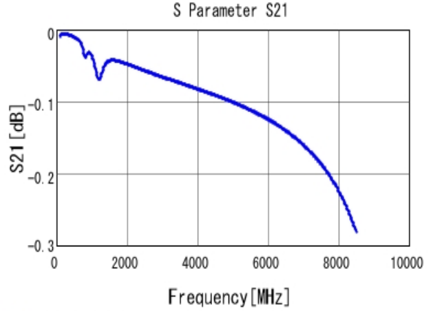
■ GRM1555C1H471GA01 S21 DCOV, 25degC
