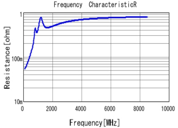
■ GRM1555C1H471GA01 R DCOV, 25degC
