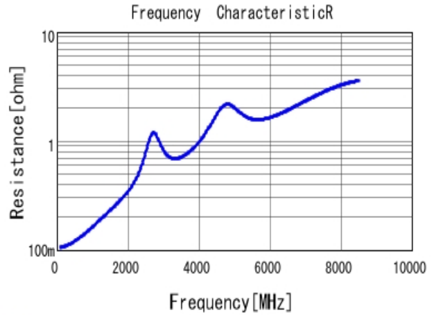
■ GRM1555C1H430JA01 R DCOV, 25degC
