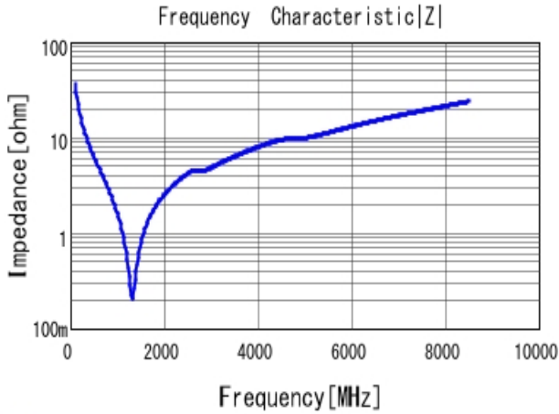
■ GRM1555C1H430JA01 |Z| DCOV, 25degC
