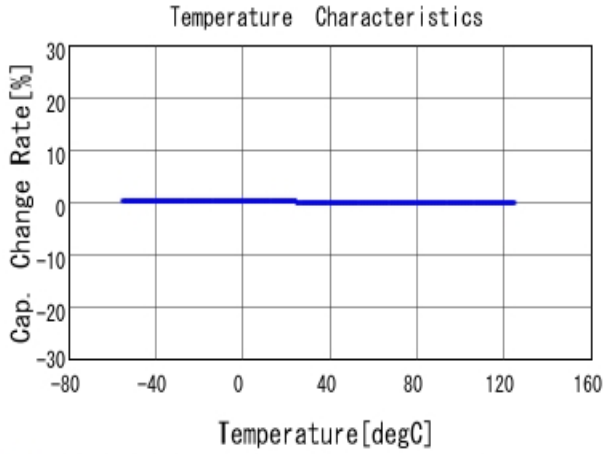
■ GRM1555C1H430JA01 C-Temp. capchange, DCOV, AC1Vrms
