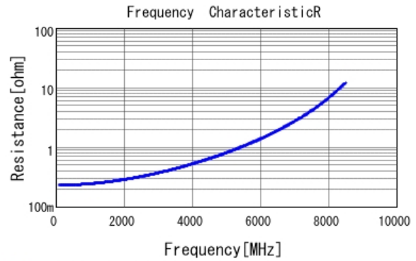
■ GRM1555C1H3R9CA01 R DCOV, 25degC
