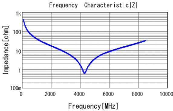
■ GRM1555C1H3R9CA01 |Z| DCOV, 25degC
