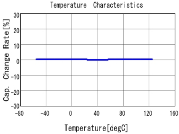
■ GRM1555C1H3R9BA01 C-Temp. capchange, DCOV, AC1Vrms
