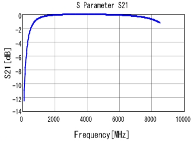
■ GRM1555C1H3R9BA01 S21 DCOV, 25degC
