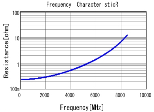
■ GRM1555C1H3R9BA01 R DCOV, 25degC
