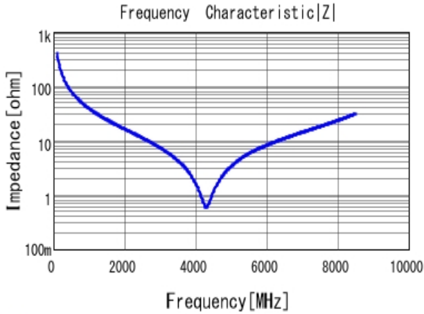
■ GRM1555C1H3R9BA01 |Z| DCOV, 25degC
