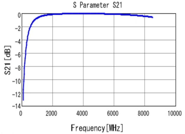
■ GRM1555C1H3R6WA01 S21 DCOV, 25degC
