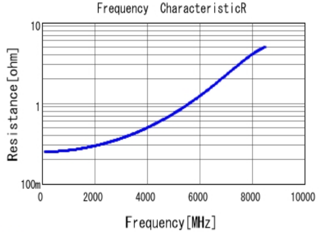
■ GRM1555C1H3R6WA01 R DCOV, 25degC
