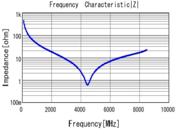
■ GRM1555C1H3R6WA01 |Z| DCOV, 25degC
