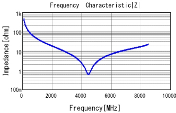
■ GRM1555C1H3R6CA01 |Z| DCOV, 25degC
