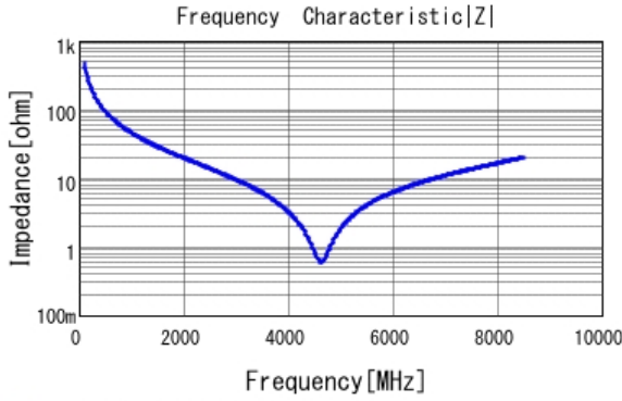
■ GRM1555C1H3R3BA01 |Z| DCOV, 25degC
