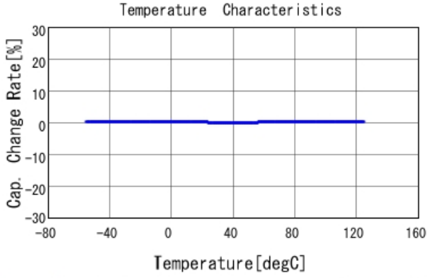
GRM1555C1H3R0CA01 C-Temp. capchange, DCOV, AC1Vrms
