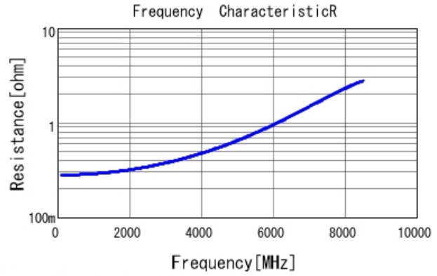
GRM1555C1H3R0CA01 R DCOV, 25degC
