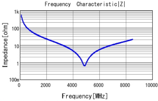
GRM1555C1H3R0CA01 |Z| DCOV, 25degC
