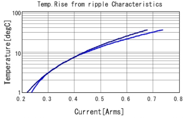
GRM1555C1H3R0CA01 Temp. rise — 2GHz — 3GHz
