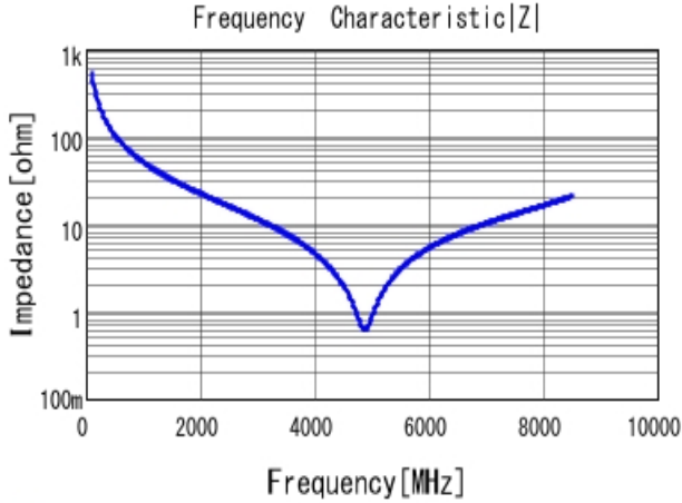
■ GRM1555C1H3R0BA01 |Z| DCOV, 25degC
