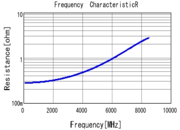
■ GRM1555C1H3R0BA01 R DCOV, 25degC
