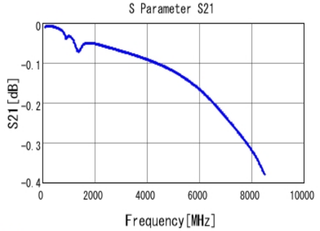
■ GRM1555C1H391JA01 S21 DCOV, 25degC
