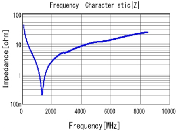
■ GRM1555C1H390JA01 |Z| DC0V, 25degC
