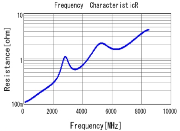
■ GRM1555C1H390JA01 R DC0V, 25degC
