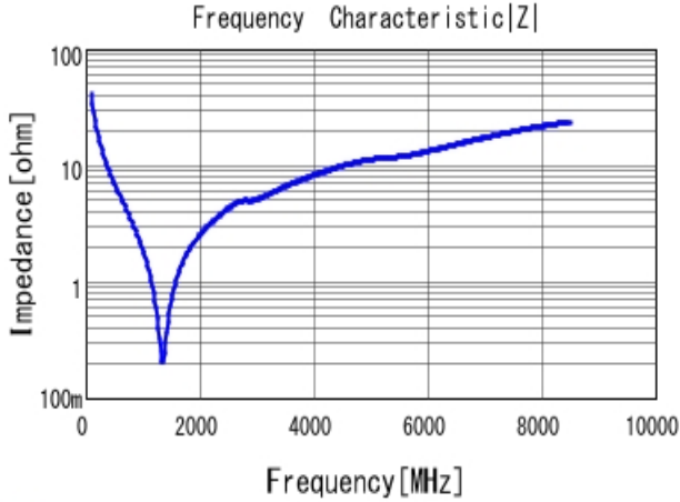
■ GRM1555C1H390GA01 |Z| DCOV, 25degC
