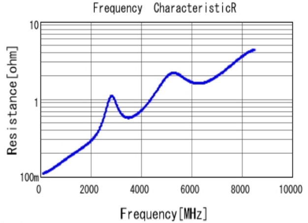
■ GRM1555C1H390GA01 R DCOV, 25degC
