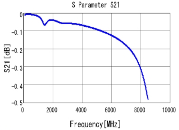
■ GRM1555C1H361JA01 S21 DCOV, 25degC
