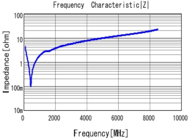
■ GRM1555C1H361JA01 |Z| DCOV, 25degC
