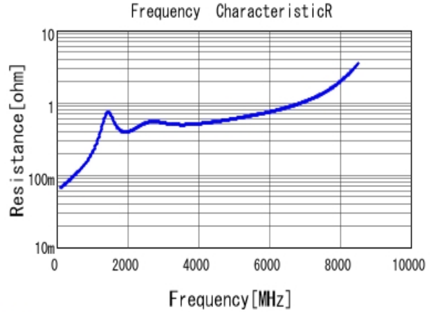
■ GRM1555C1H361JA01 R DCOV, 25degC
