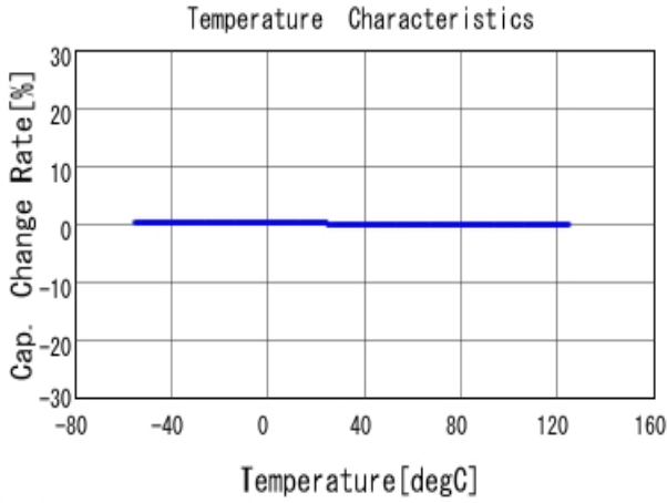
■ GRM1555C1H361JA01 C-Temp. capchange, DCOV, AC1Vrms
