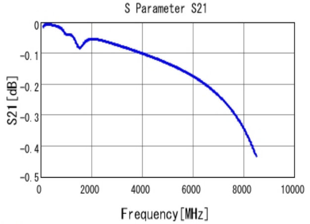
■ GRM1555C1H331JA01 S21 DCOV, 25degC
