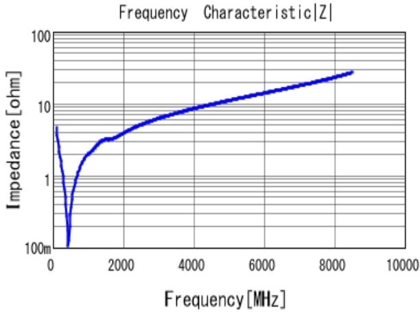
■ GRM1555C1H331JA01 |Z| DC0V, 25degC
