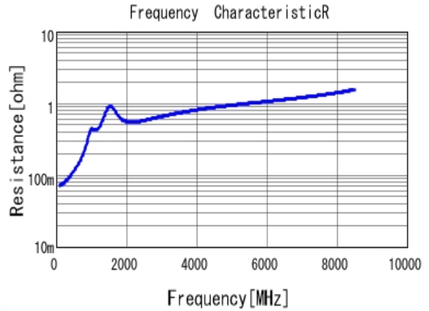
■ GRM1555C1H331JA01 R DC0V, 25degC
