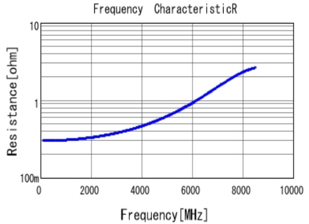
■ GRM1555C1H2R7WA01 R DCOV, 25degC
