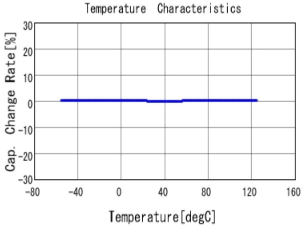
■ GRM1555C1H2R7WA01 C-Temp. capchange, DCOV, AC1Vrms
