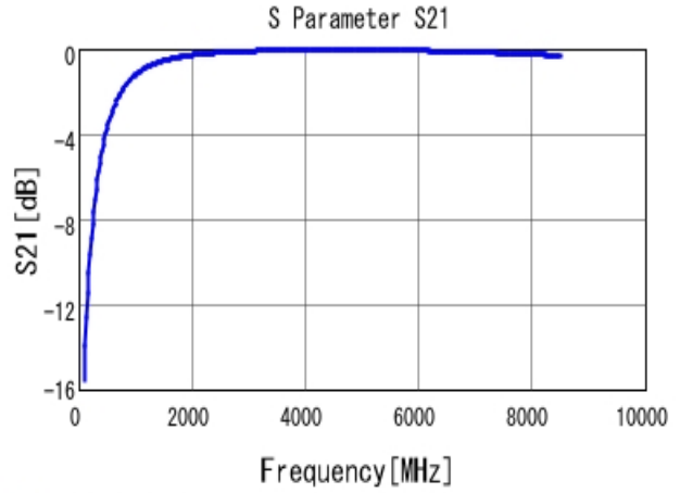
■ GRM1555C1H2R7WA01 S21 DCOV, 25degC
