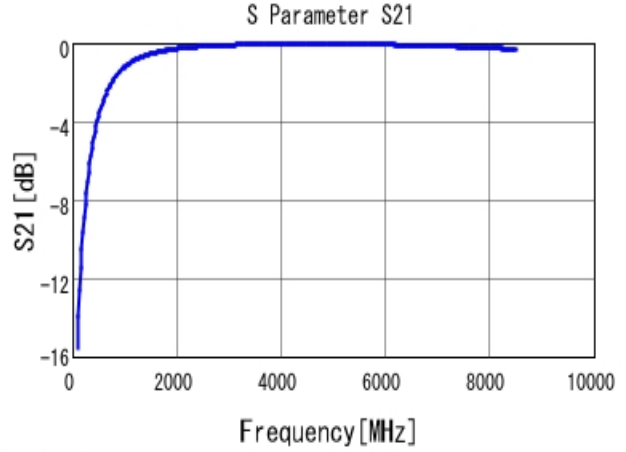
■ GRM1555C1H2R7CA01 S21 DCOV, 25degC
