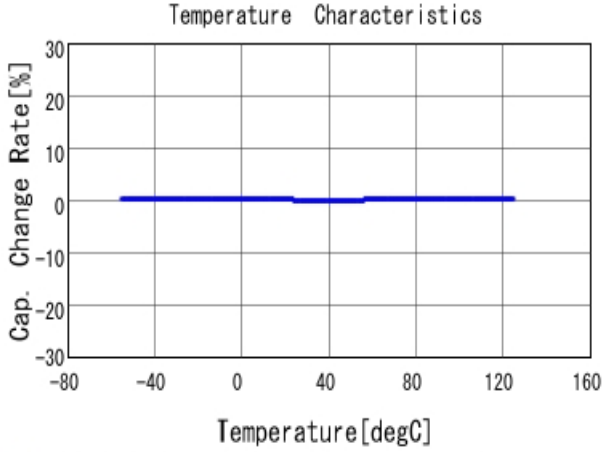
■ GRM1555C1H2R7CA01 C-Temp. capchange, DCOV, AC1Vrms
