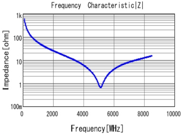
■ GRM1555C1H2R7CA01 |Z| DC0V, 25degC
