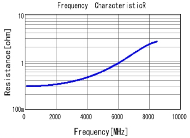
■ GRM1555C1H2R7BA01 R DC0V, 25degC
