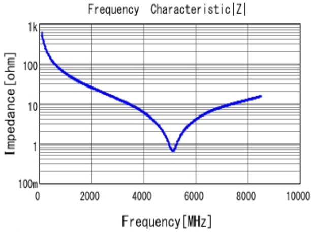
■ GRM1555C1H2R7BA01 |Z| DC0V, 25degC
