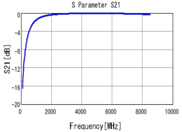
■ GRM1555C1H2R4BA01 S21 DCOV, 25degC
