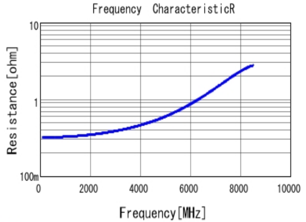
■ GRM1555C1H2R4BA01 R DC0V, 25degC
