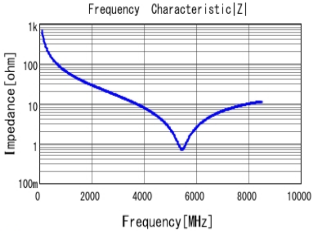
■ GRM1555C1H2R4BA01 |Z| DC0V, 25degC
