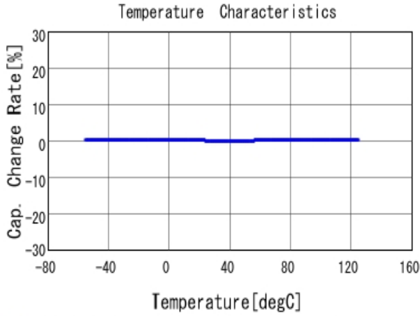
■ GRM1555C1H2R4BA01 C-Temp. capchange, DCOV, AC1Vrms
