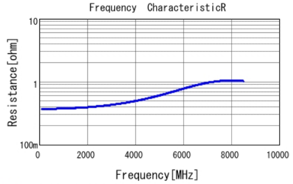
■ GRM1555C1H2R2BA01 R DCOV, 25degC
