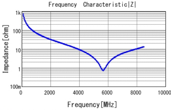
■ GRM1555C1H2R2BA01 |Z| DCOV, 25degC
