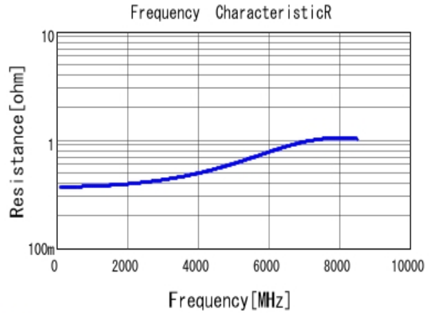
■ GRM1555C1H2R0CA01 R DCOV, 25degC
