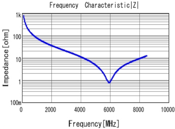
■ GRM1555C1H2R0CA01 |Z| DCOV, 25degC
