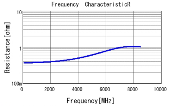
■ GRM1555C1H2R0BA01 R DCOV, 25degC
