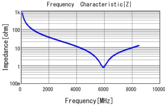
■ GRM1555C1H2R0BA01 |Z| DCOV, 25degC
