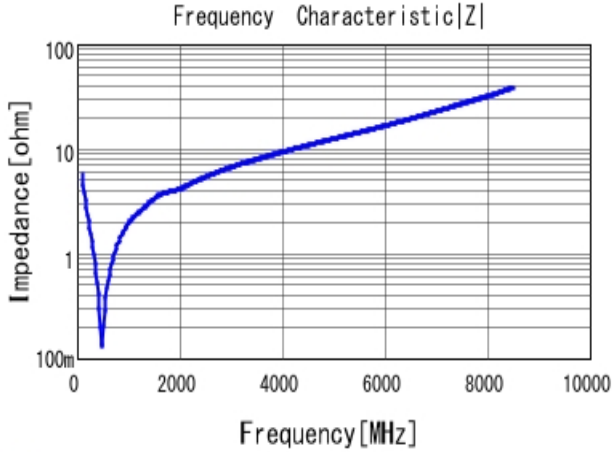
■ GRM1555C1H271GA01 |Z| DC0V, 25degC
