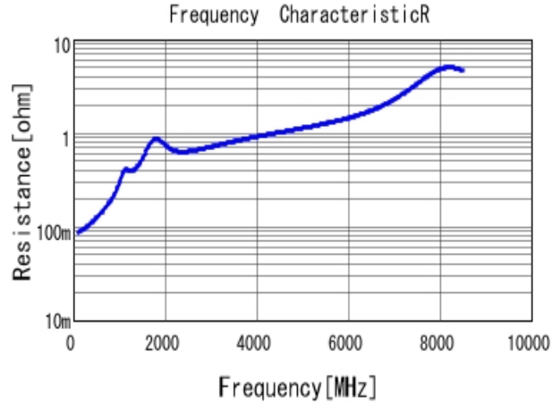
■ GRM1555C1H271GA01 R DC0V, 25degC
