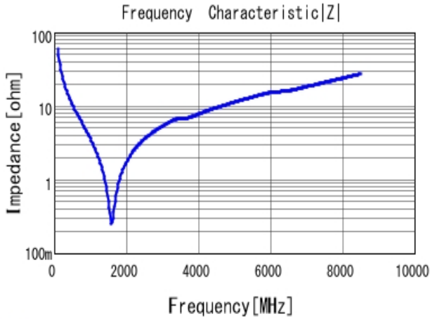
■ GRM1555C1H270GA01 |Z| DCOV, 25degC
