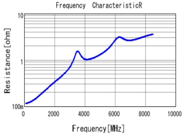
■ GRM1555C1H270GA01 R DCOV, 25degC
