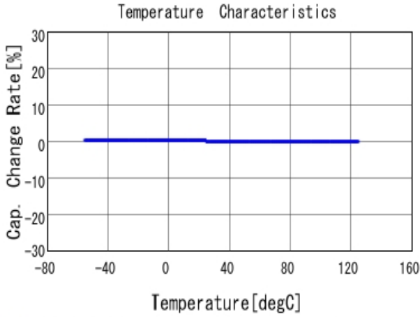
■ GRM1555C1H270GA01 C-Temp. capchange, DCOV, AC1Vrms
