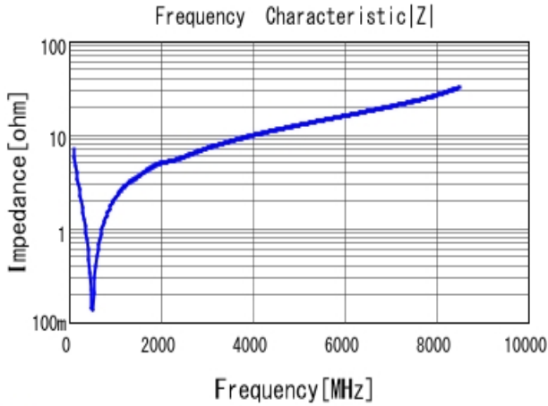
■ GRM1555C1H221JA01 |Z| DCOV, 25degC
