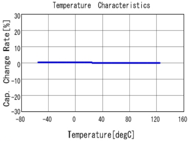
■ GRM1555C1H221JA01 C-Temp. capchange, DCOV, AC1Vrms
