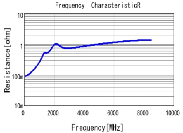
■ GRM1555C1H221JA01 R DCOV, 25degC
