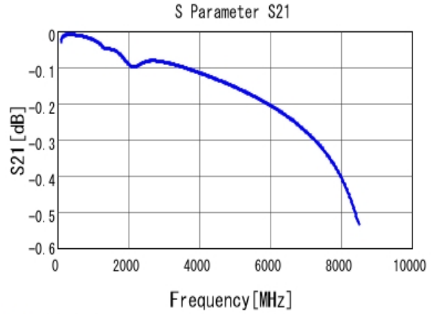
■ GRM1555C1H221JA01 S21 DCOV, 25degC
